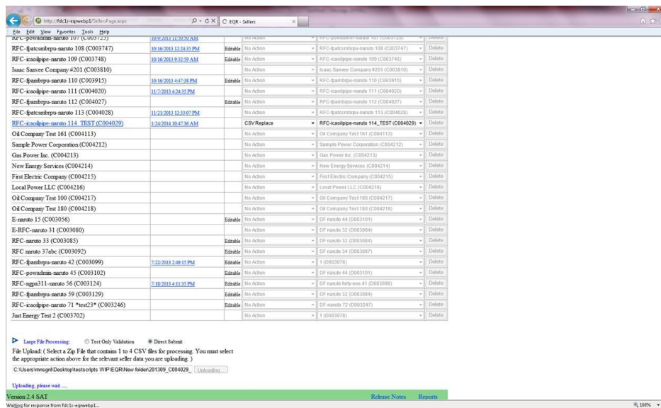
Figure 5 – Uploading Process
